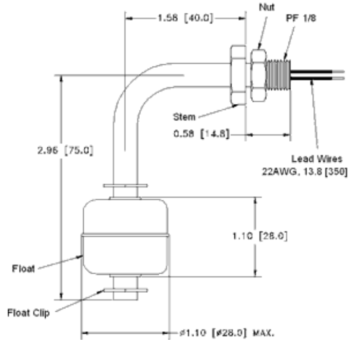
Dimensions: Inches [mm]
